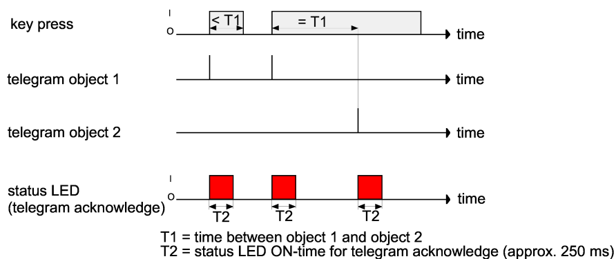
Figure 17: Example of "object 1 and object 2" operating concept
