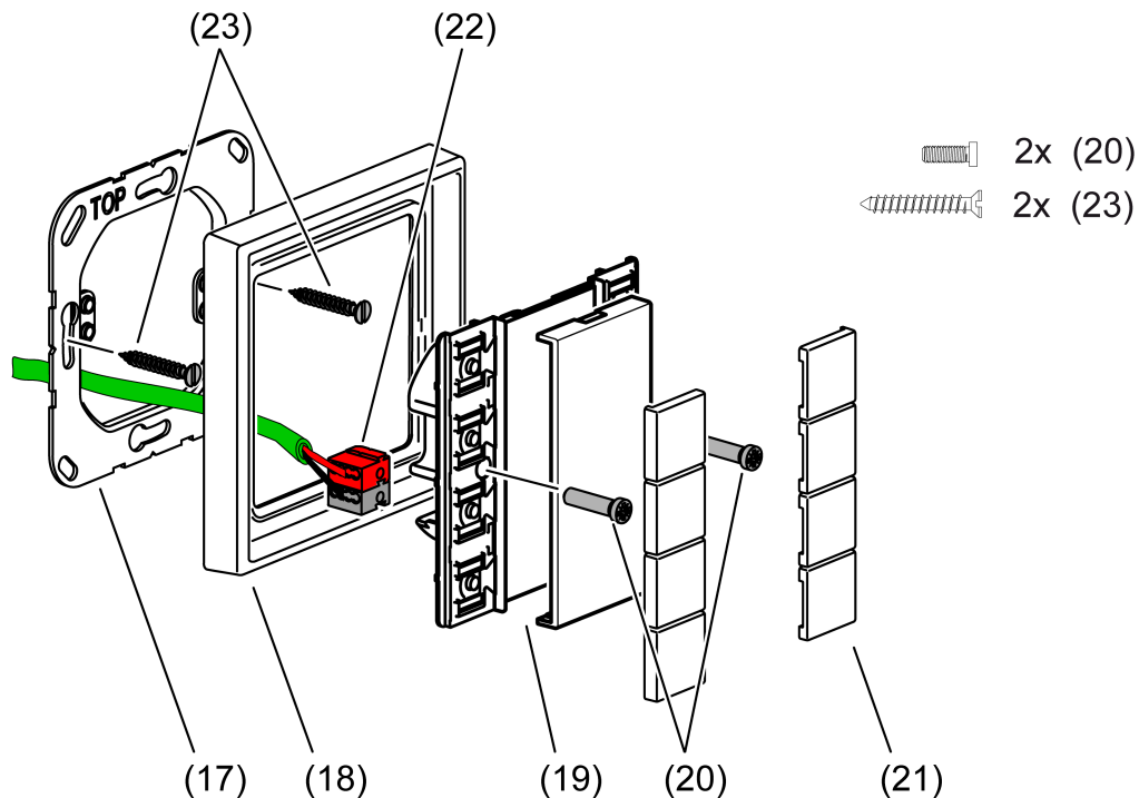
Figure 5: Mounting the push-button sensor basic module
