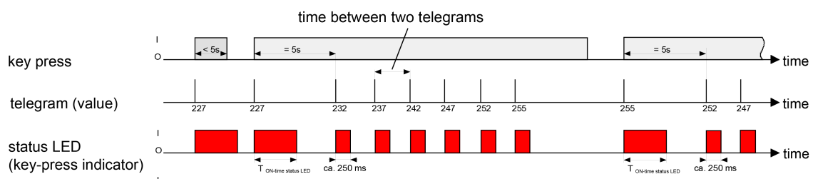
Figure 14: Example of value adjustment without value range overflow
