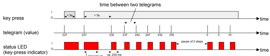
Figure 15: Example of value adjustment with value range overflow
