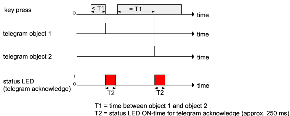
Figure 16: Example of "object 1 or object 2" operating concept
