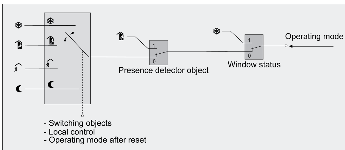
Figure 54: Operating mode change-over through 4 x 1-bit objects with presence detector
