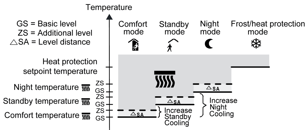
Figure 60: Setpoint temperatures in the operating mode "Basic and additional cooling" (recommended specification)
