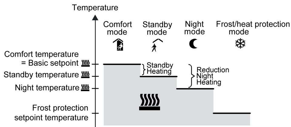
Figure 57: Setpoint temperatures in the operating mode "Heating" (recommended specification)
