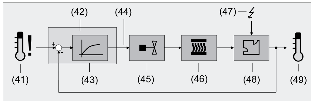
Figure 44: Controlled system of single-room temperature control
