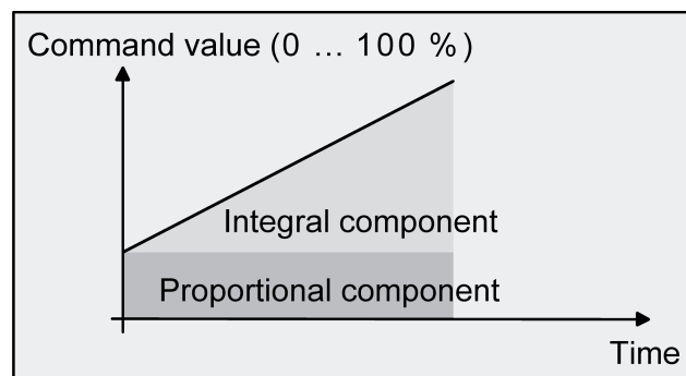
Figure 45: Continuous PI control
