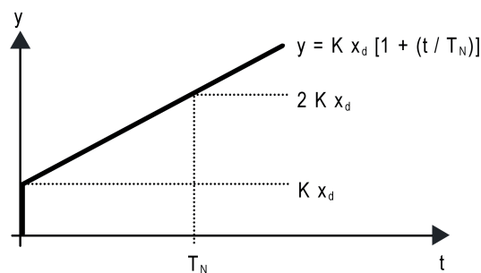
Figure 51: Function of the command value of a PI control
