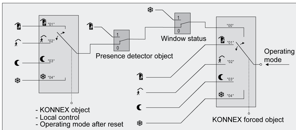
Figure 56: Operating mode change-over through KONNEX object with presence detector
