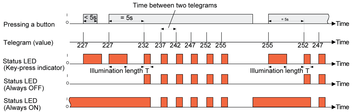
Figure 40: Example of value adjustment without value range overflow
