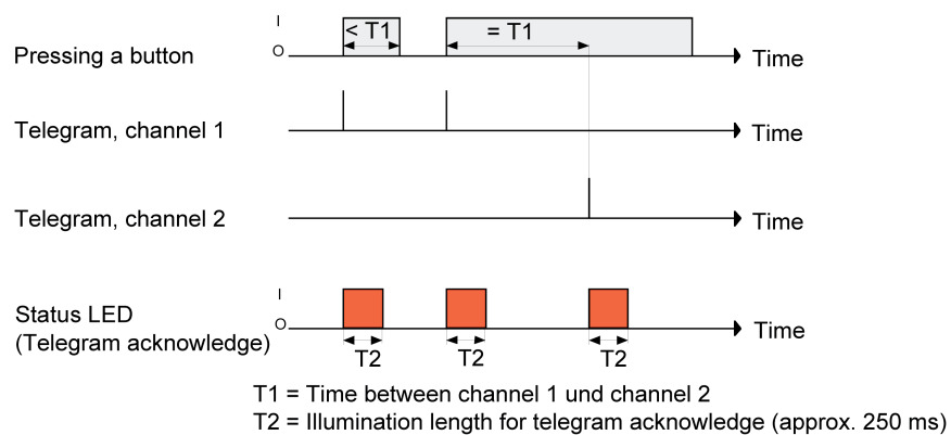
Figure 43: Example for operation concept "Channel 1 and channel 2"
