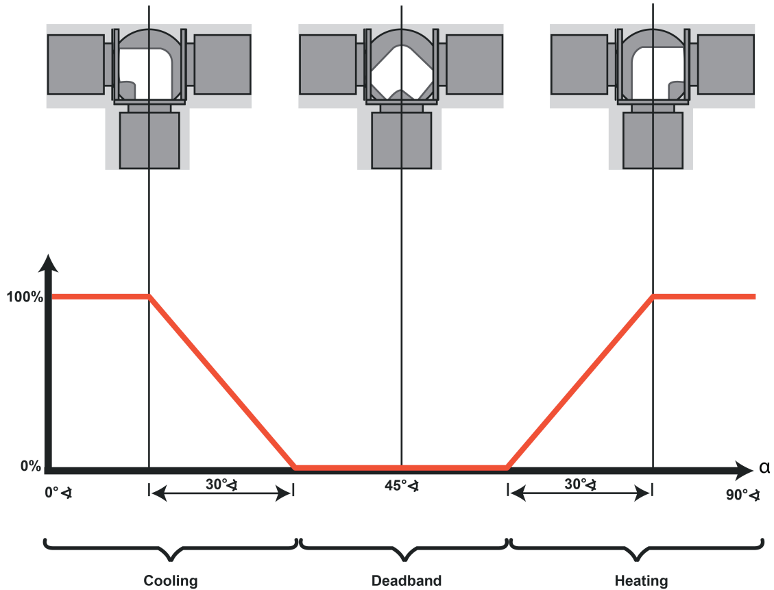
Figure 65: Control ball valve - valve curve
