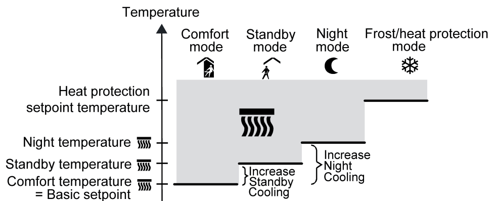
Figure 59: Setpoint temperatures in the operating mode "Cooling" (recommended specification)
