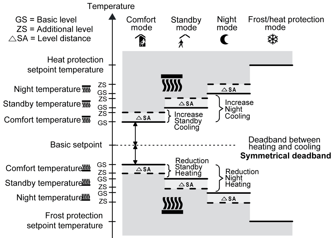
Figure 63: Setpoint temperatures in the operating mode "Basic and additional heating and cooling" with symmetrical deadband (recommended specification)
