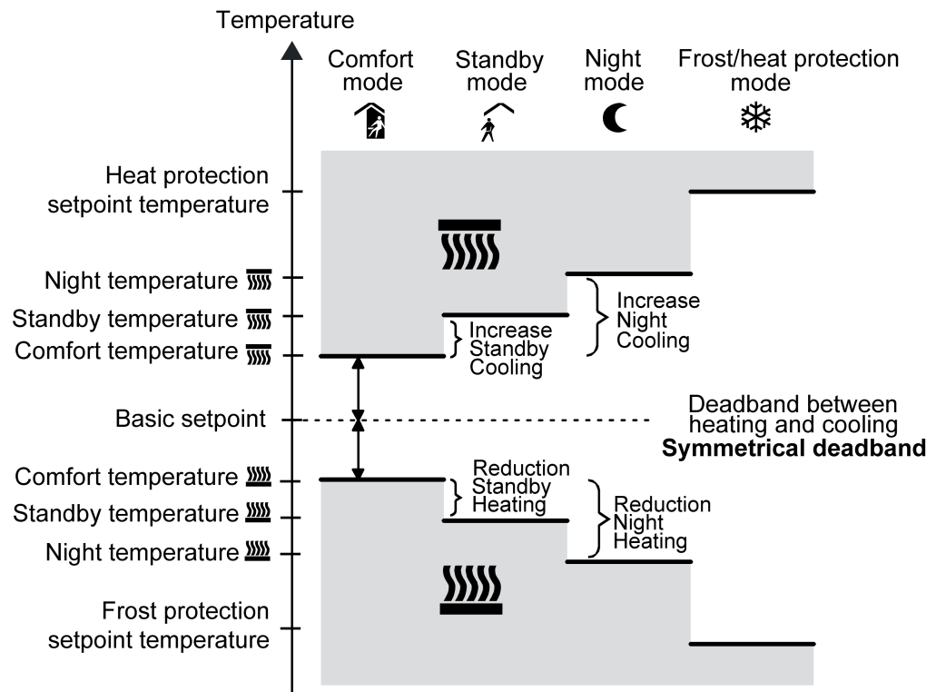
Figure 61: Setpoint temperatures in the operating mode "Heating and cooling" with symmetrical deadband (recommended specification)
