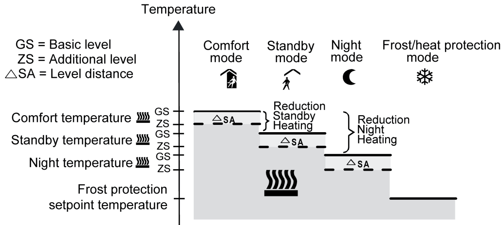
Figure 58: Setpoint temperatures in the operating mode "Basic and additional heating" (recommended specification)
