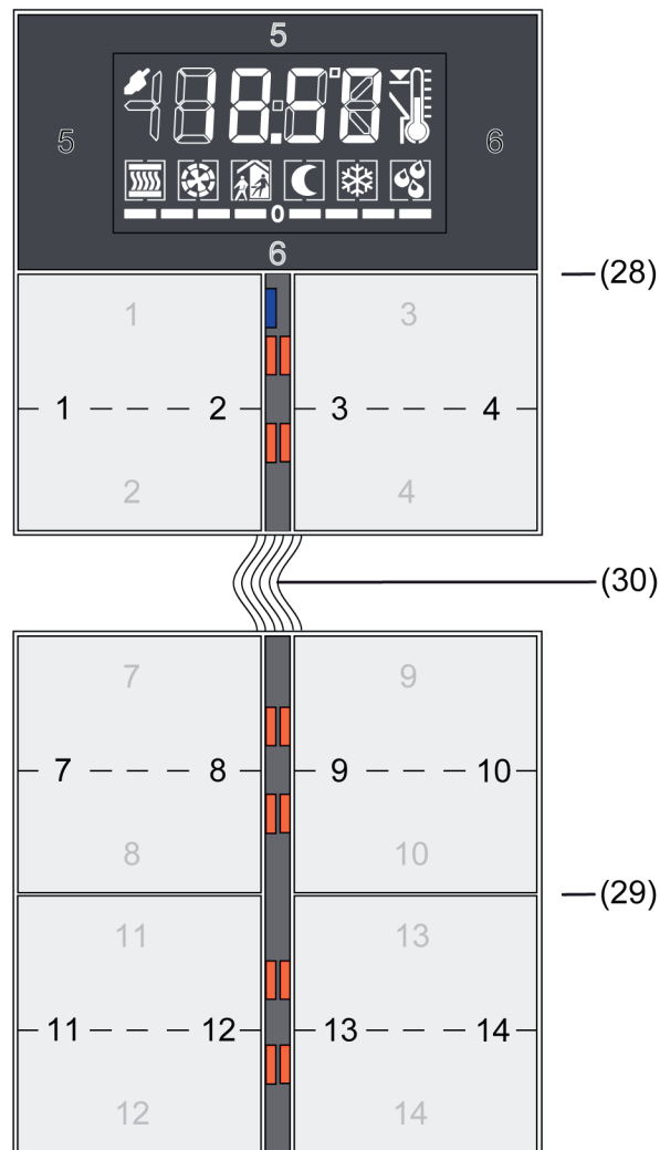
Figure 28: Example of button pair/control surface numbering in connection with a 4gang extension module
