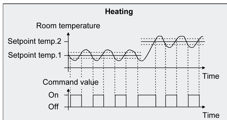
Figure 47: 2-point feedback control for the single "Heating" operating mode
