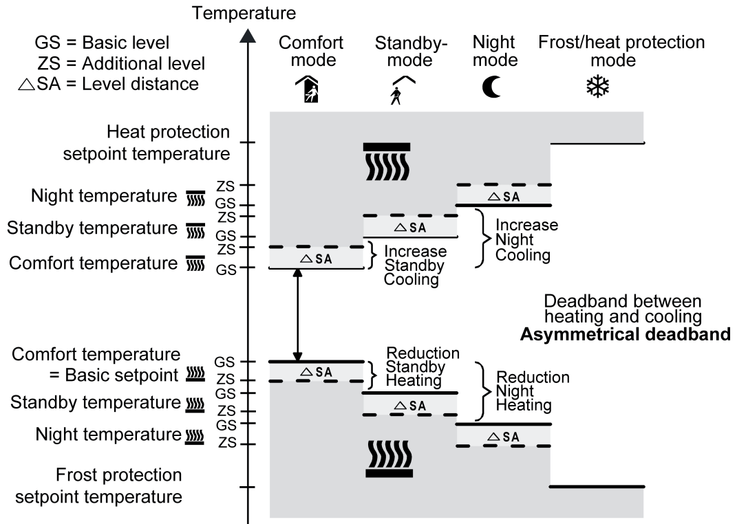
Figure 64: Setpoint temperatures in the operating mode "Basic and additional heating and cooling" with asymmetrical deadband (recommended specification)
