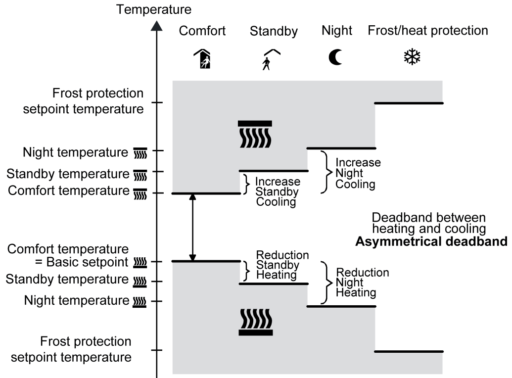
Figure 62: Setpoint temperatures in the operating mode "Heating and cooling" with asymmetrical deadband (recommended specification)
