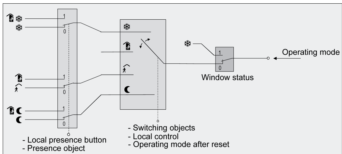
Figure 53: Operating mode change-over through 4 x 1-bit objects with presence button
