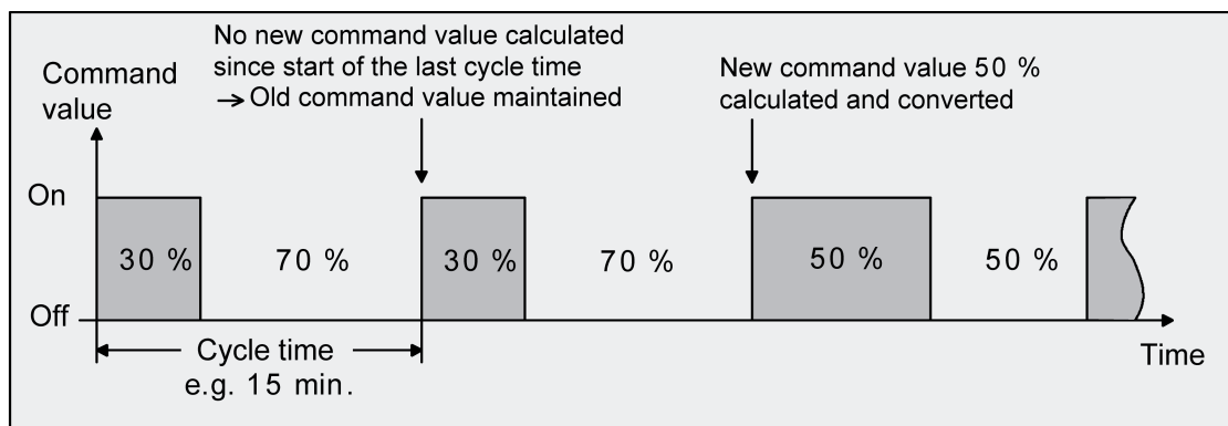
Figure 46: Switching PI control
