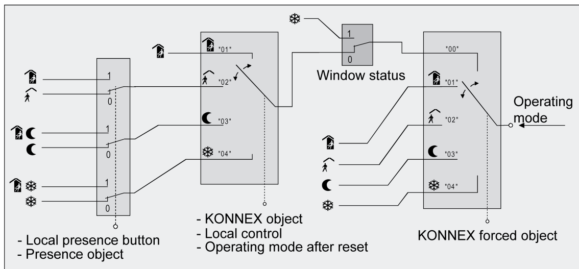
Figure 55: Operating mode change-over through KONNEX object with presence button
