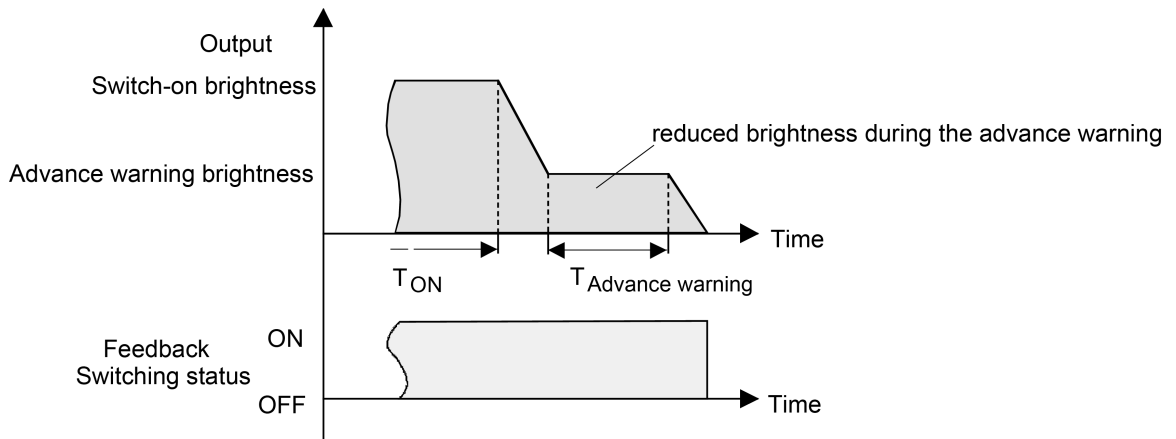
Image 21: The pre-warning function of the staircase function with soft OFF function (as an example with minimum brightness = 0%)
