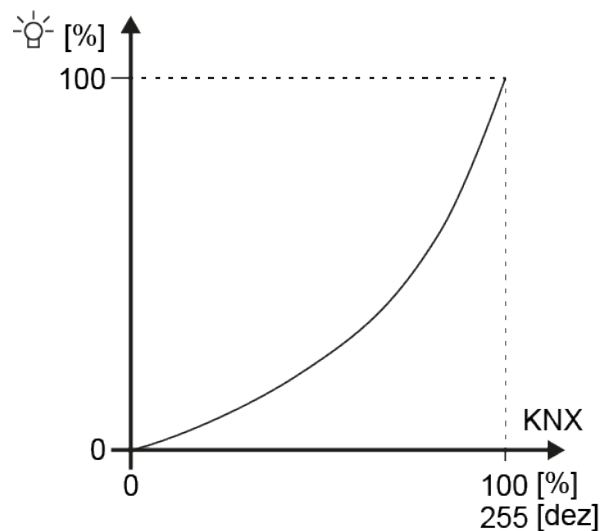
Figure 22: Combined dimming characteristic curve at the output of an operating device
