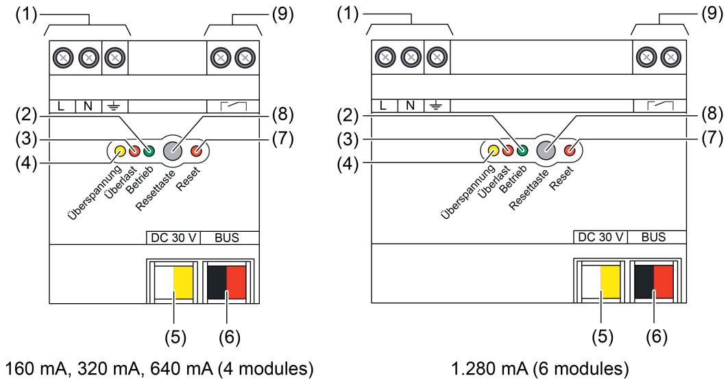
Figure 1: Device components
