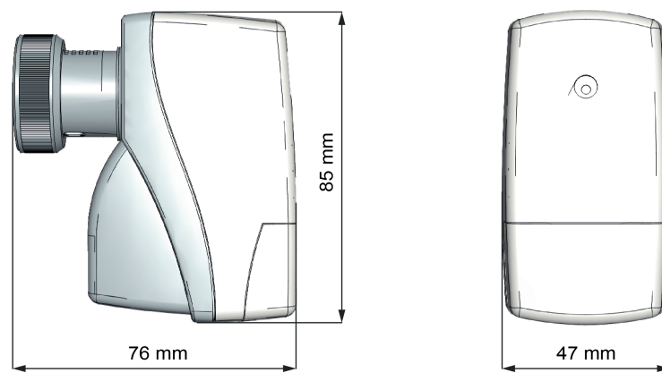
Figure 3: Device components, dimensions
