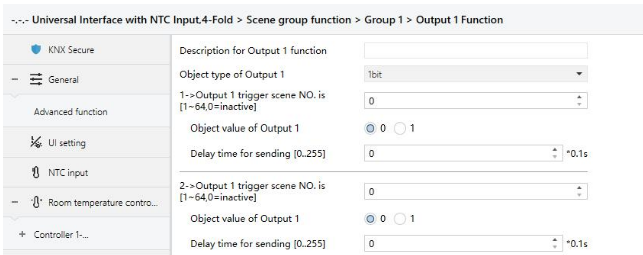
Fig.4.5(3) "Output Y function"parameter window
