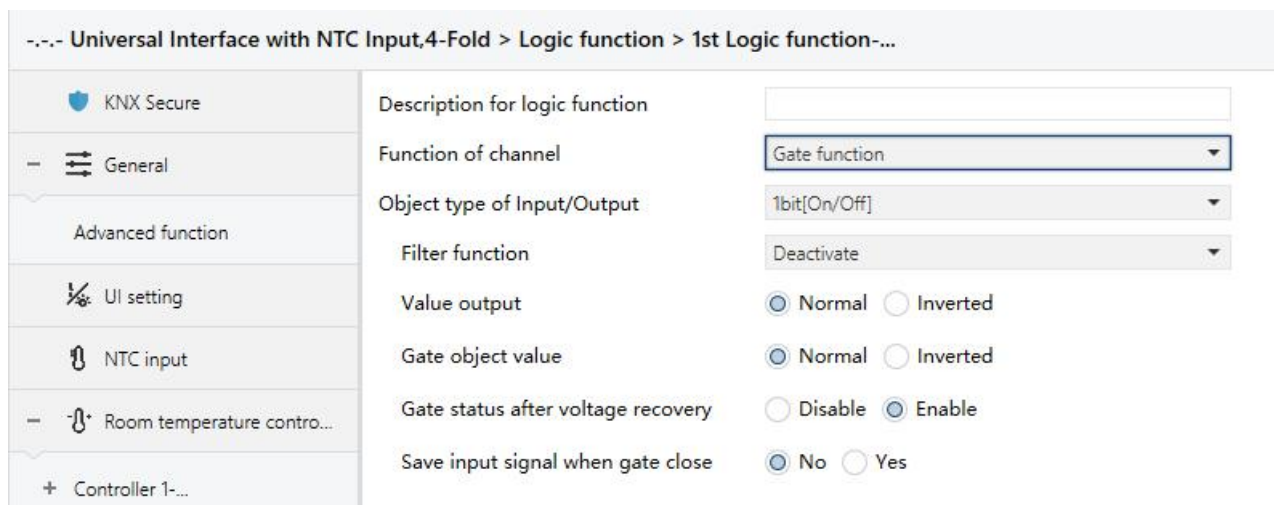
Fig.4.4.5 “Gate function”parameter window
