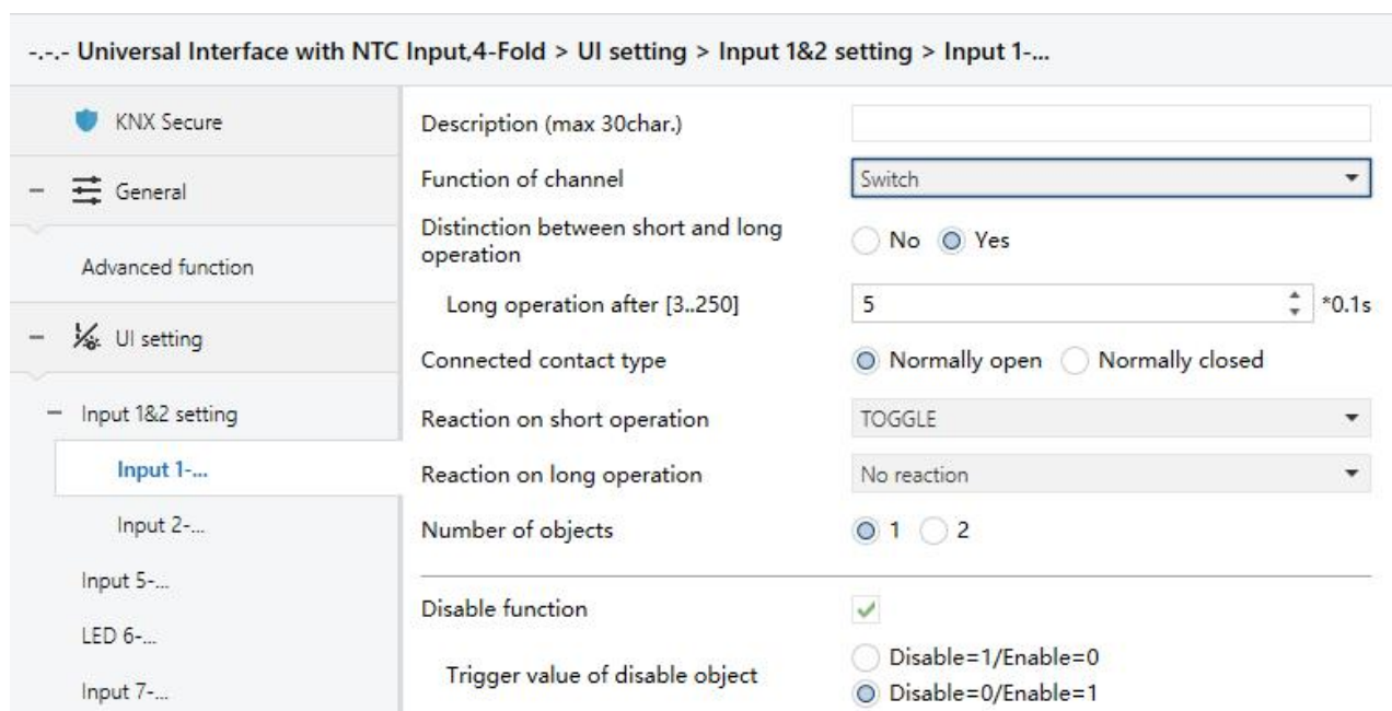
Fig.4.6.2.1parameter window “Input x-Switch”
