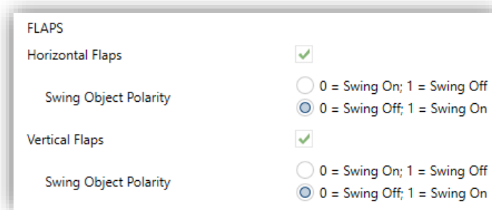
Figure 4. AC Gateway. Configuration. Flaps.
