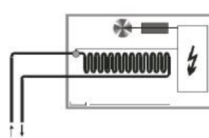
2 pipe system
