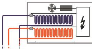
3 pipe system
