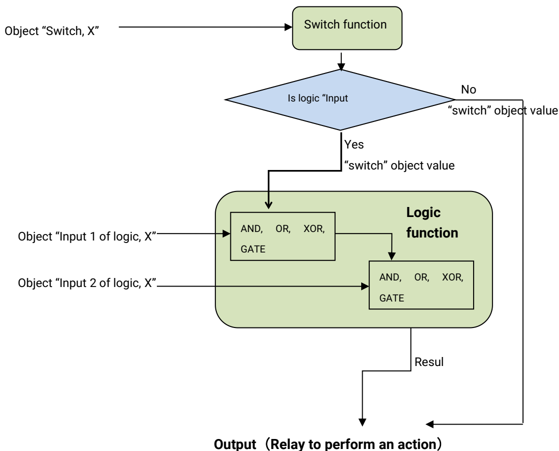
Fig. 5.15 switch and logical function diagram
