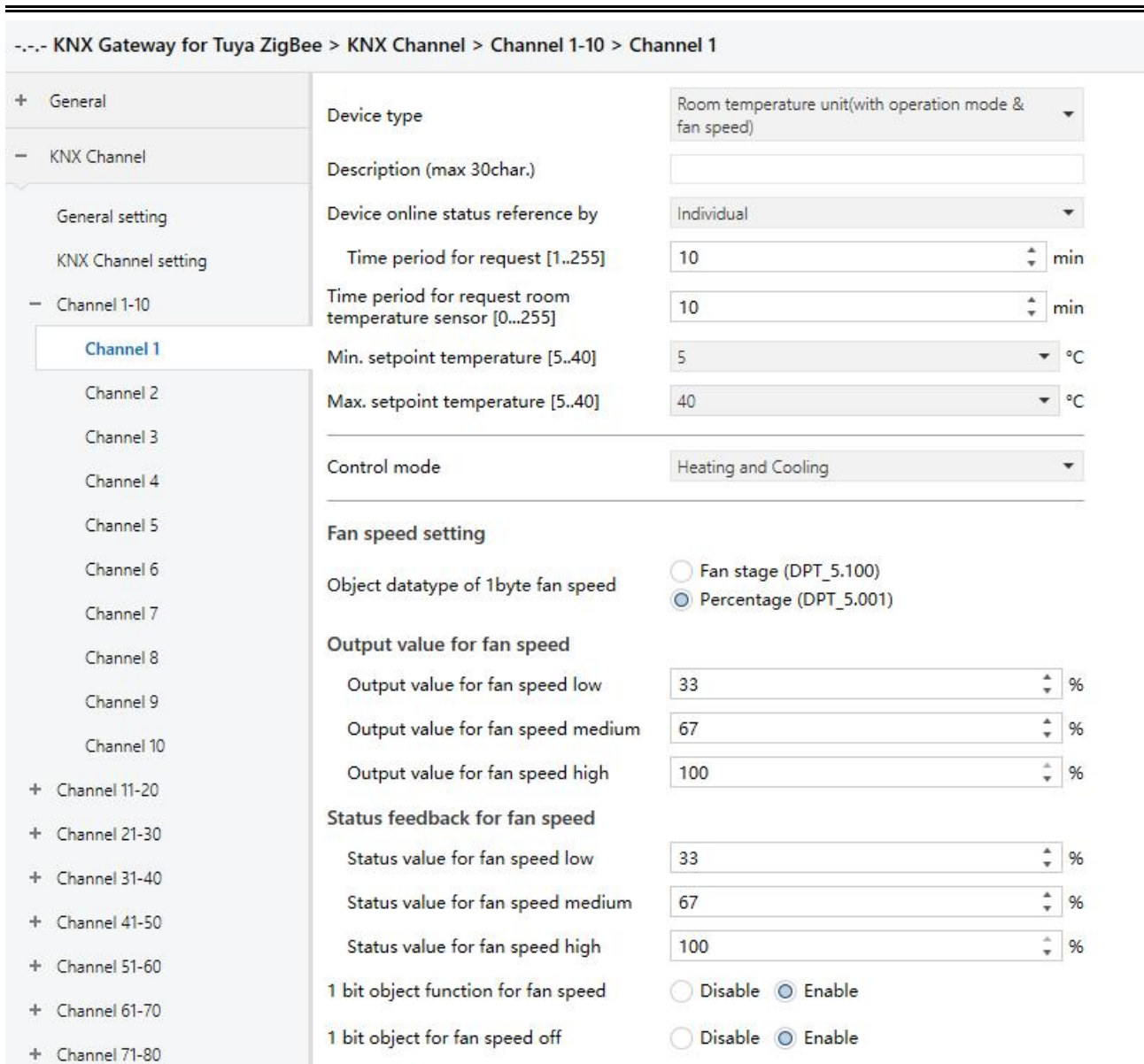
Fig.5.2.1.3 Parameter setting of room temperature unit
